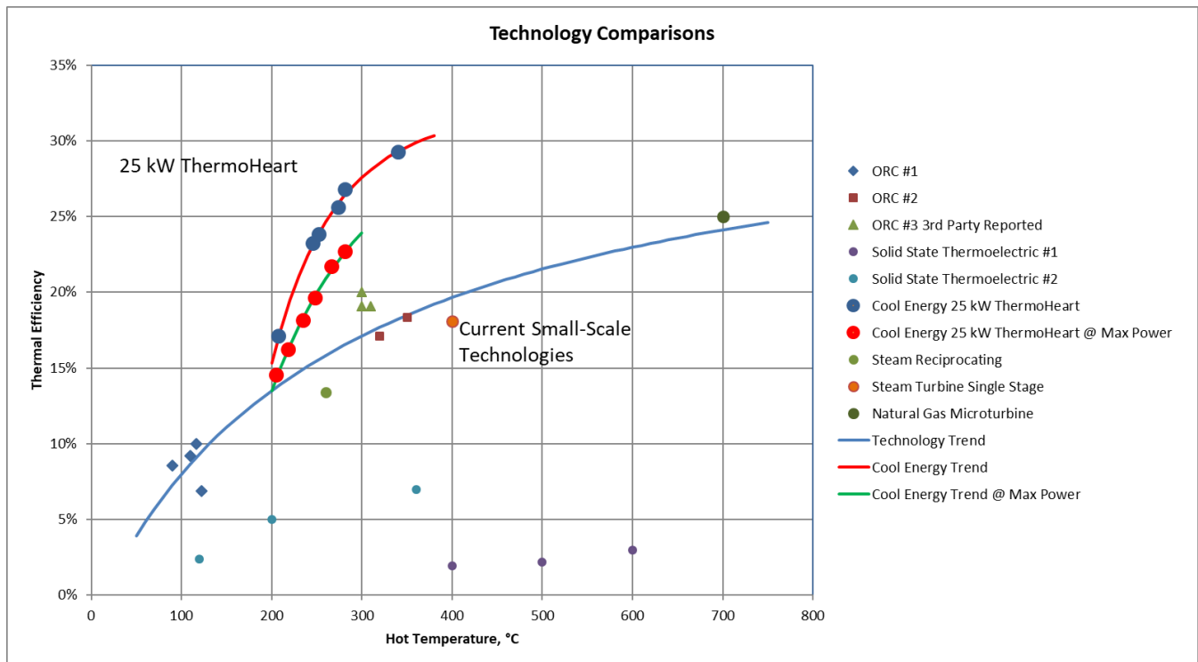
Figure 1) Chart of performance of generating technologies including the Gen 5 25kW ThermoHeart Engine, various organic Rankine cycle systems, solid state thermoelectric generators (TEGs), and steam and gas turbine systems. The blue line is the fit through all of the data except TEGs and the ThermoHeart Engine. The red line is the fit through the measured performance of the ThermoHeart Engine at maximum efficiency, and the green line is the measured ThermoHeart fit at max power.
